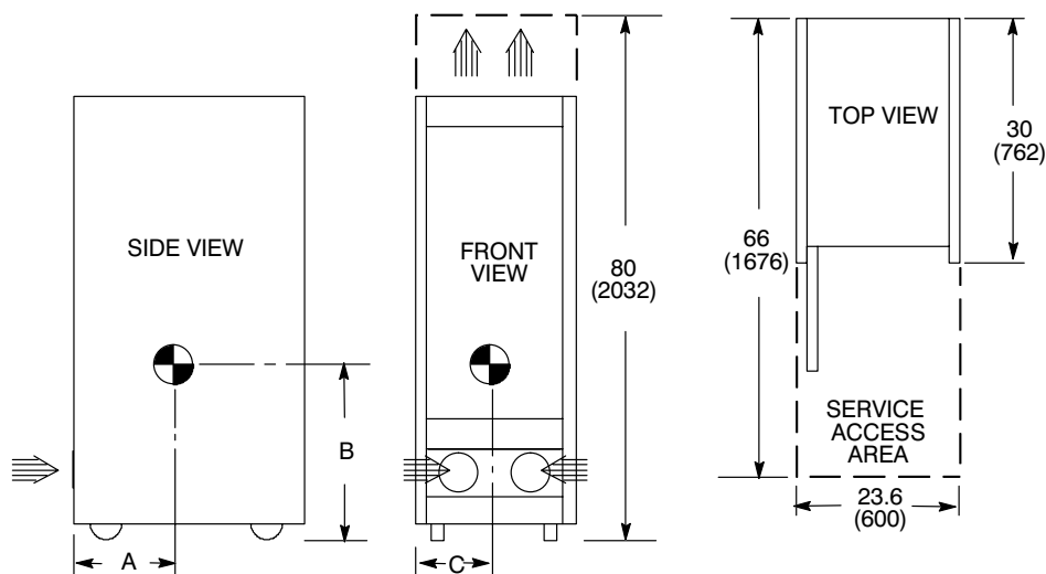
SERVICE AND VENTILATION CLEARANCE
